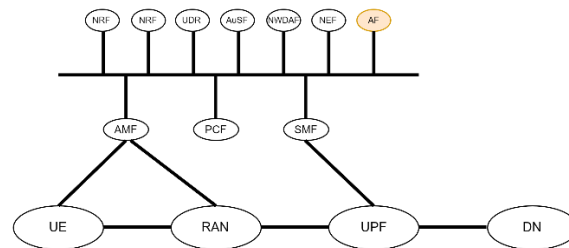
Figure 1: 5G Service Based Interfaces
